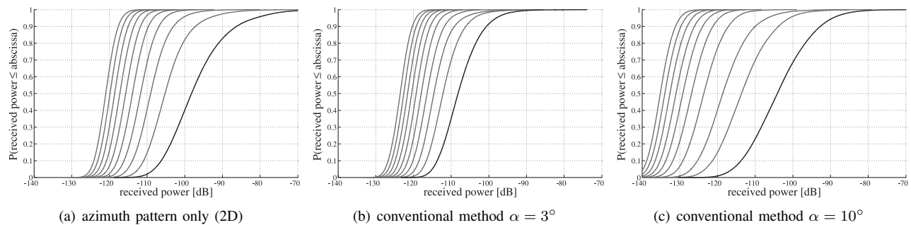
Fig. 9. Power distributions for the 10 strongest signals
