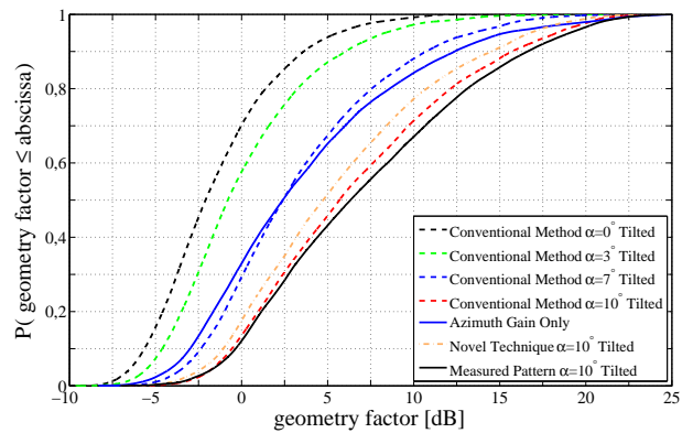
Fig. 8. User geometries obtained from multi-cell SCME simulations
