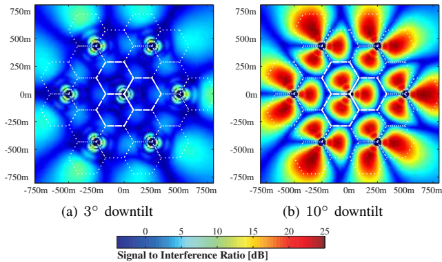
Fig. 7. SIR maps obtained from simplified multi-cell simulations
